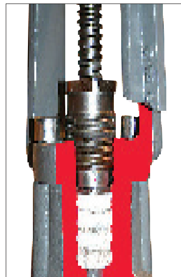
Example gland packing application.
